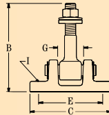
BOLT-ON BRACKET
