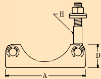
WELD-ON BRACKET
