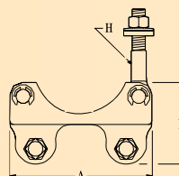
CLAMP-ON BRACKET
