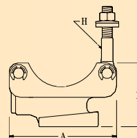
WEDGE BRACKET
