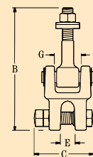
CLAMP-ON BRACKET
